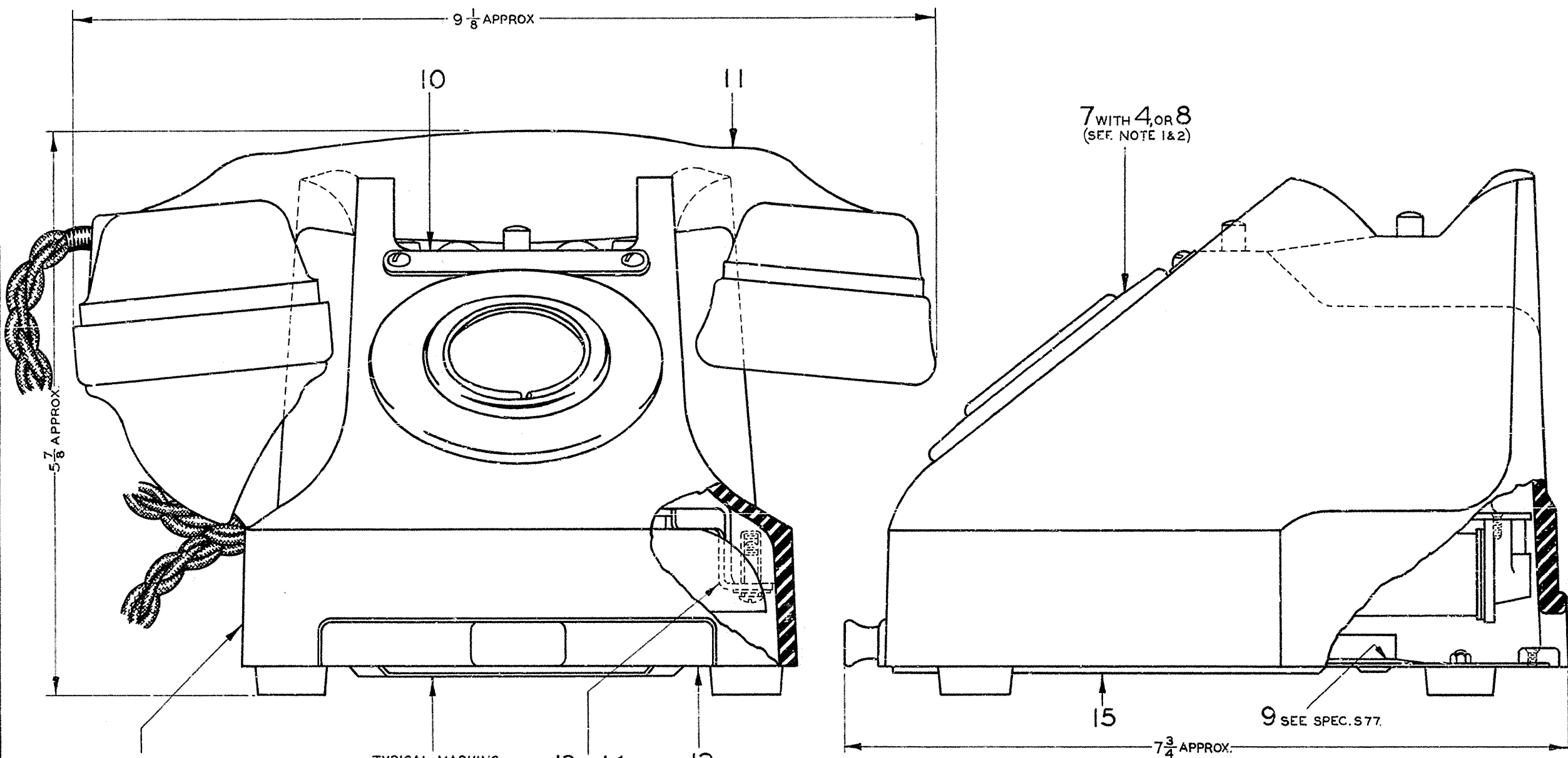
PART SECTION (WITH ITEMS 1,2,3,5,6,12 & 13 OMITTED)
