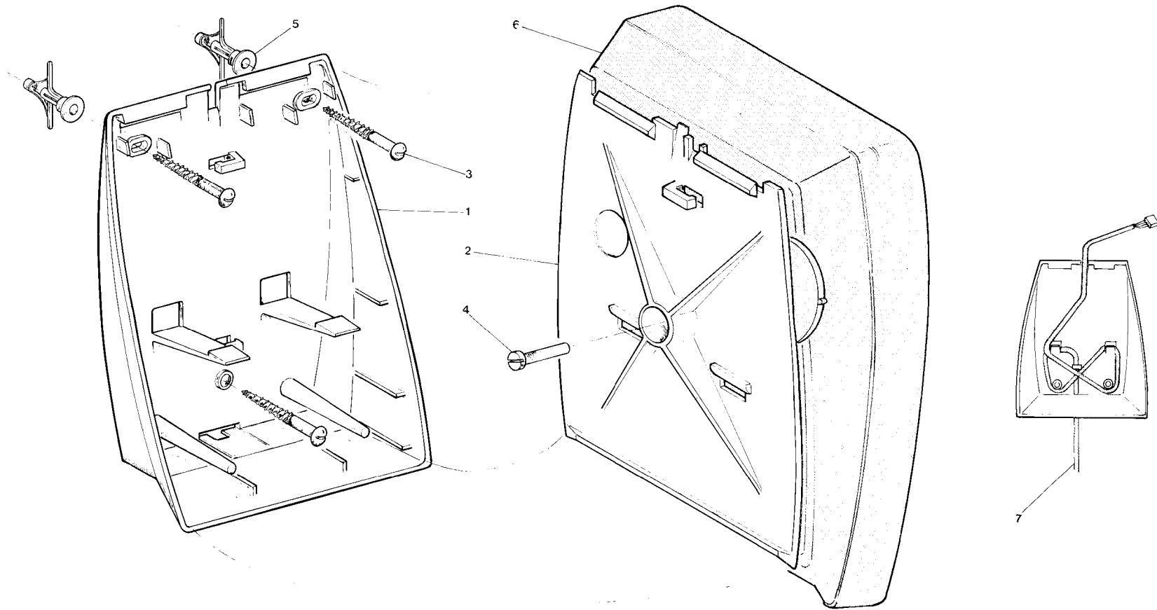
1.WALL PLATE, 2.BASE PLATE, 3.No 8 WOODSCREW, 4. SCREW (from telephone), 5.WALL PLUG, 6. IXT TELEPHONE, 7. LINE CORD.
