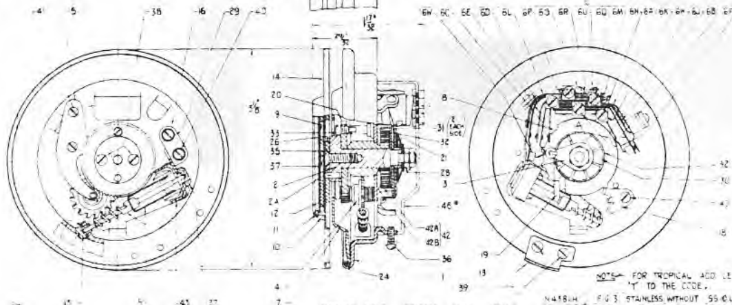
FRONT VIEW WITH FINGER PLATE A NUMBER RING REMOVED.
