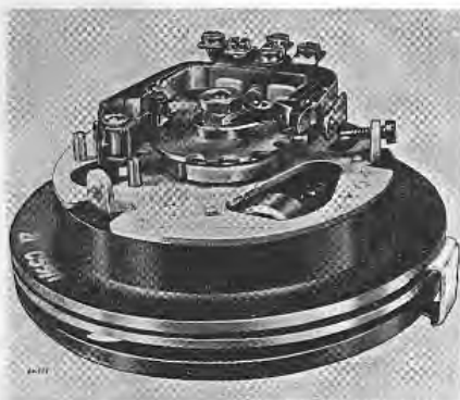
FIG. 16.—MOULDED BODY DIAL—REAR VIEW
