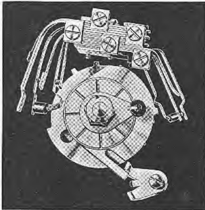
FIG. 5.—SLIPPING-CAM MECHANISM— DIAL WOUND-UP FOR DIGIT '5'
