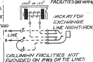
FIG. 4. PRIVATE WIRE OR TIE LINE WITHOUT EXCHANGE FACILITIES (SEE NOTE 4)
