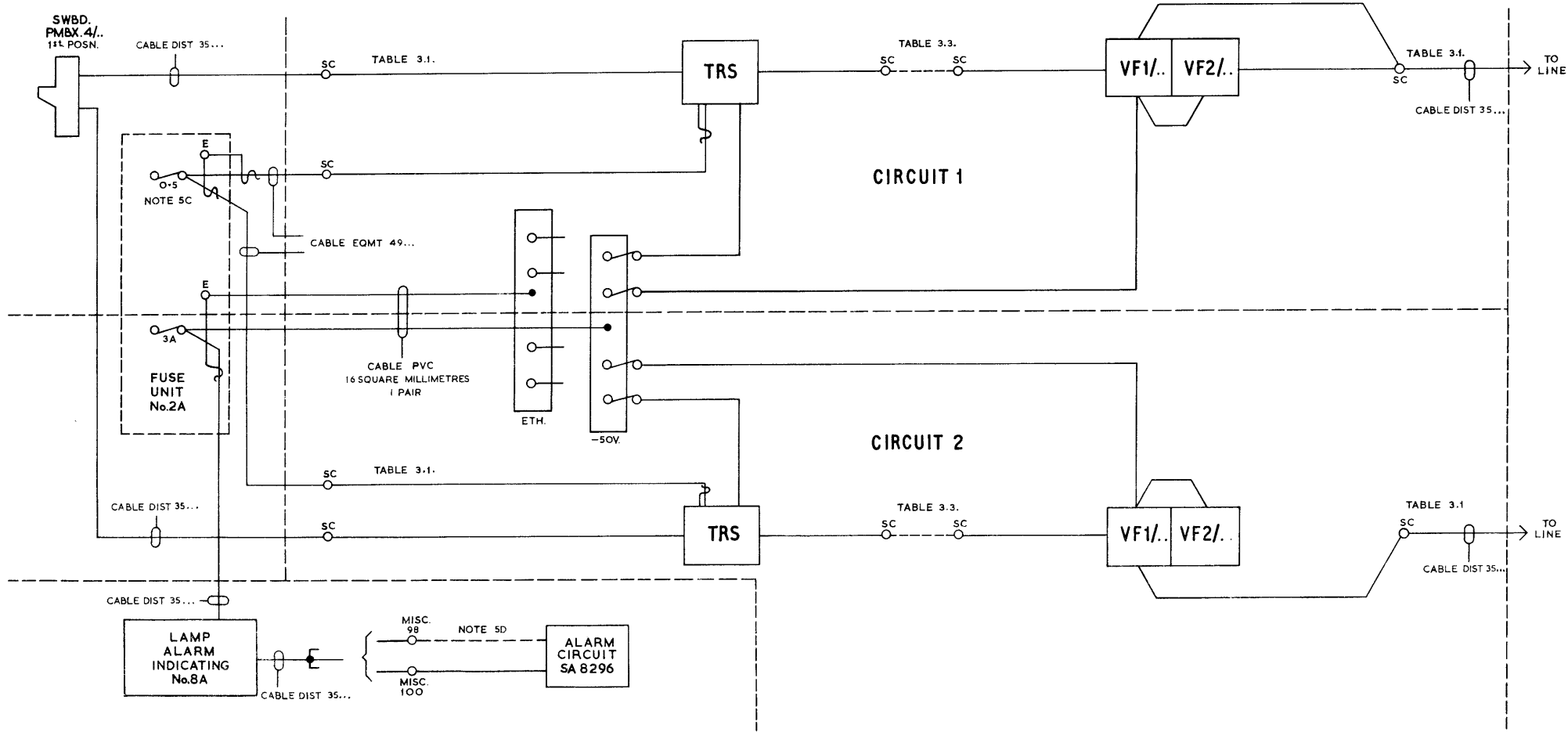
FIG. 1.2 . CABLING ARRANGEMENTS.
