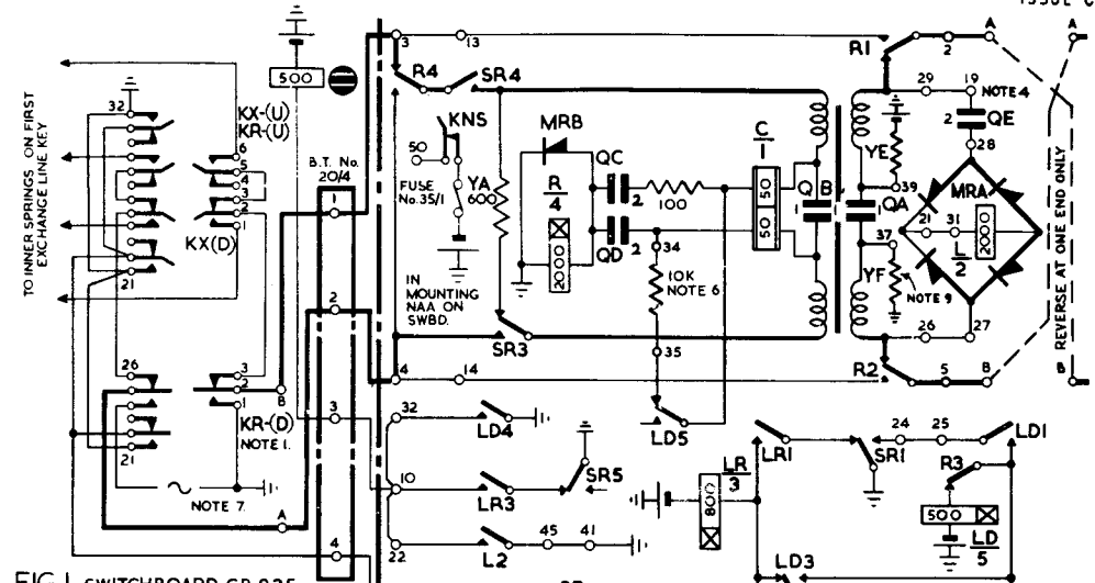
FIG. 1. SWITCHBOARD CB 935
