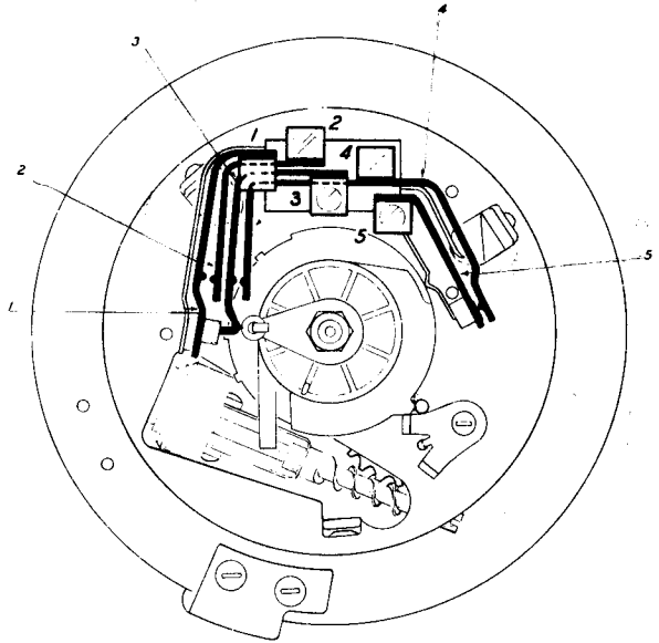
REAR VIEW SHOWING SPRING CONNEXIONS
