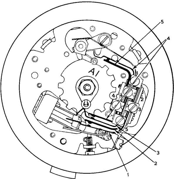
REAR VIEW SHOWING NUMBERING OF CONTACT SPRINGS AND TERMINALS
