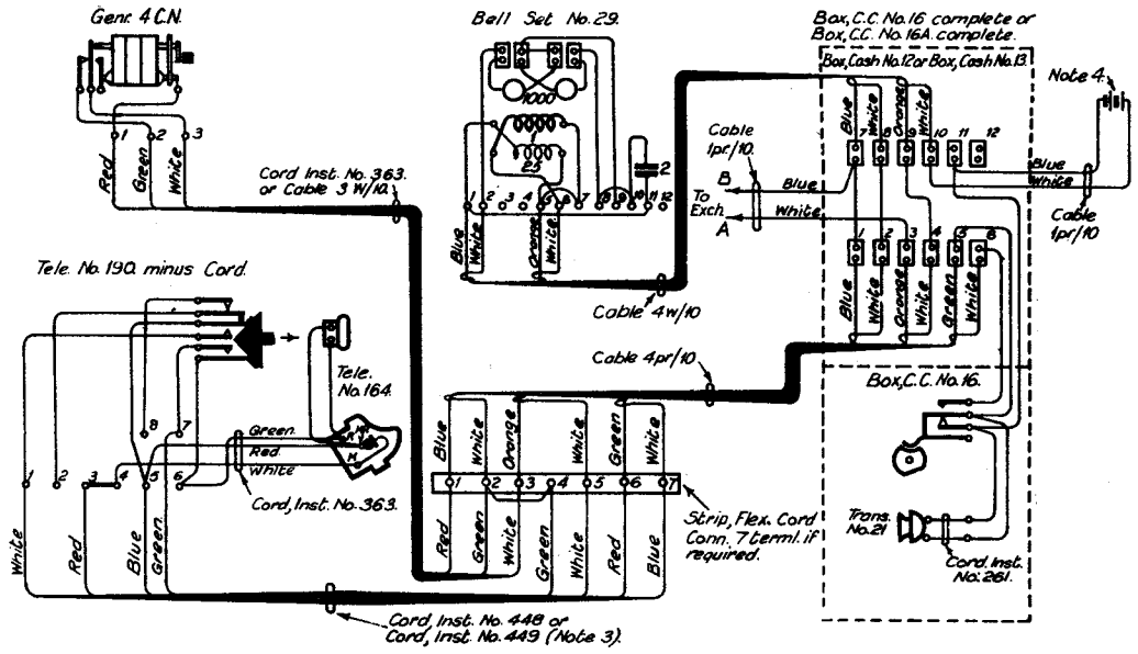
Wiring Diagram for Magneto System.
