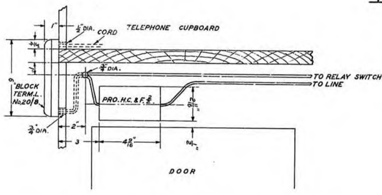
PART SECTION D-D SCALE: 1/4
